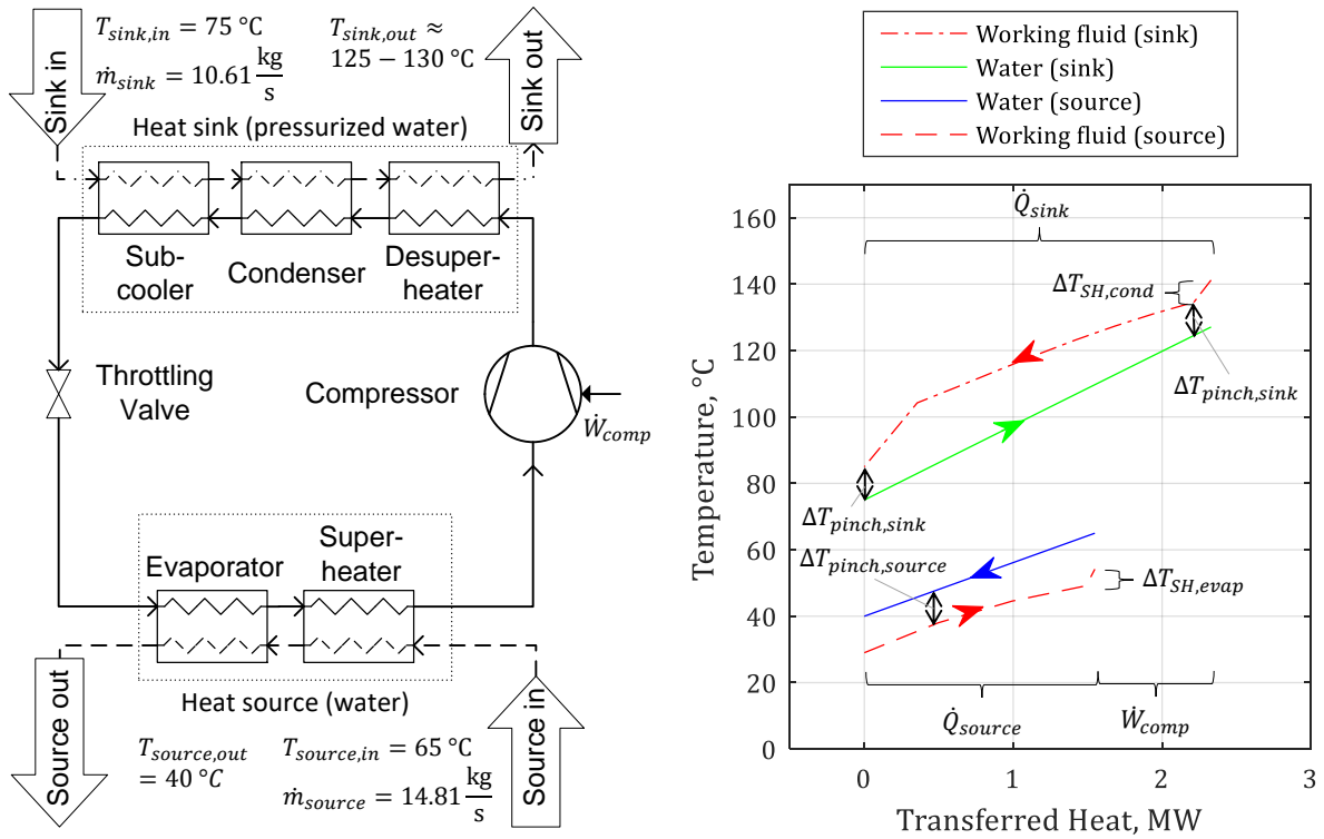
Figure 2: Flow sheet (left) and T-Q-Diagram of heat pump model with an illustrative mixture profile (right)
