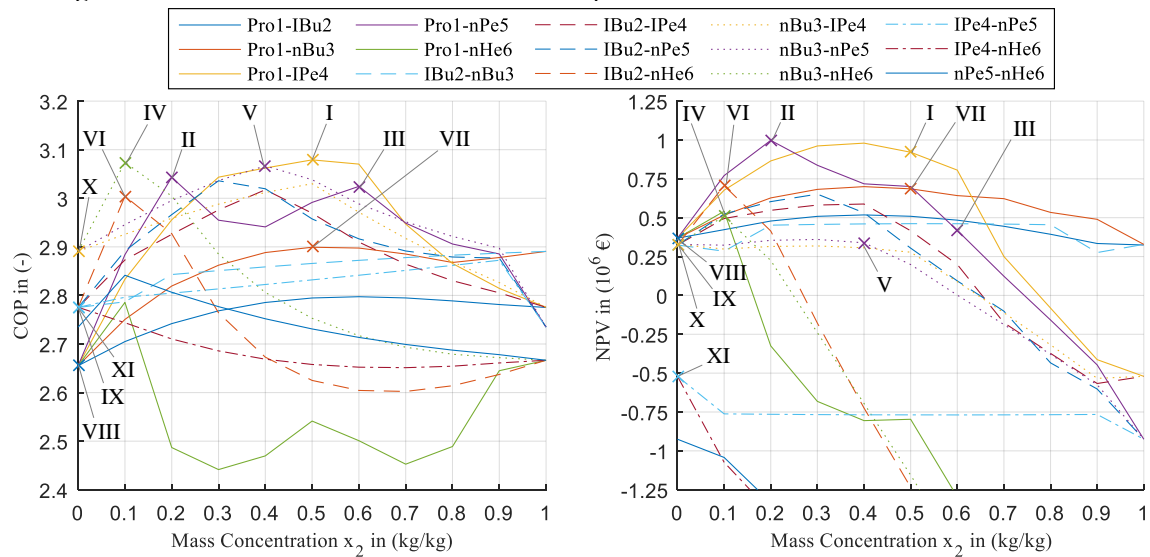
Figure 3: COP (left) and NPV (right) for all simulations. Interesting cases are marked with roman numerals (I-XI). The legend corresponds to the combination of fluids in Table 4.
