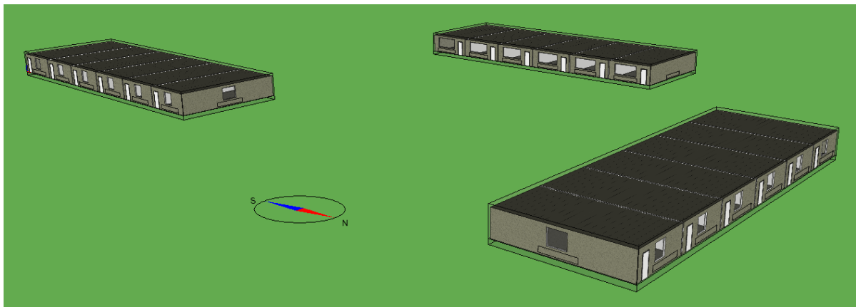
Fig. 4. The main geometry of the studied row houses modelled in the IDA ICE simulation environment.
